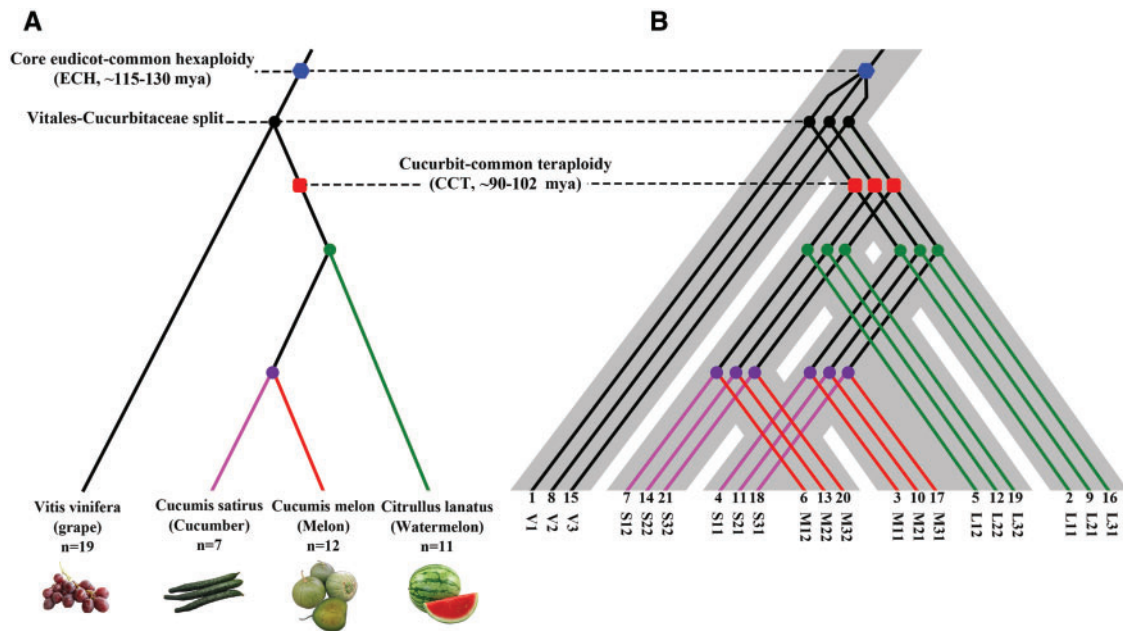
Fig. 2. Species and gene phylogenetic trees for three cucurbits. (A) Phylogenetic tree of melon (M), watermelon (L), cucumber (S), and grape (V): Eudicot-common hexaploidy (ECH) denoted by blue hexagon, cucurbit-common tetraploidy (CCT) denoted by red square; (B) Gene phylogeny: three paralogous genes in the grape genome are denoted by V1, V2, and V3 produced by the ECH, and each has two orthologs and four outparalogs in a Cucurbit genome (e.g., V1 has two orthologs M11 and M12, and four outparalogs M21, M22, M31, and M32 in melon). The species tree is produced based on our present analysis of homologous genes.
